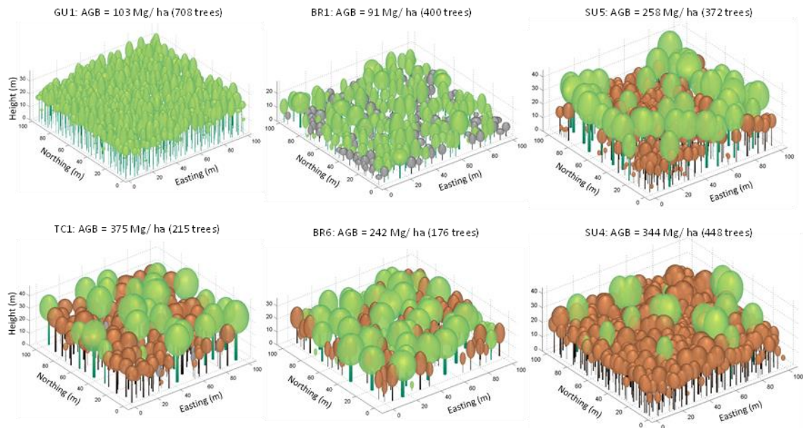
Figure 8: Examples 3D forest scene (mock-ups) of forest stands from contrasting mangrove ecosystems in the Amazon-influenced (South America).
