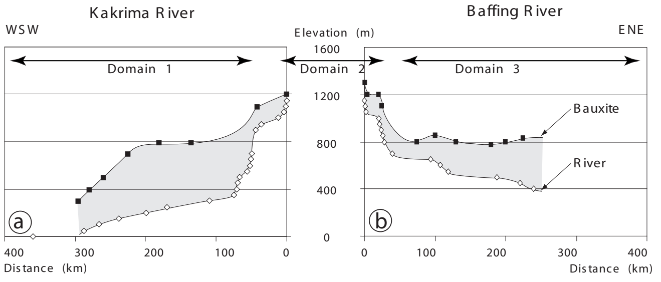
Fig. 3. Longitudinal profiles of the Kakrima (a) and Baffing (b) rivers and corresponding bauxite-capped interfluvies. River courses are shown on Fig. 2b.
