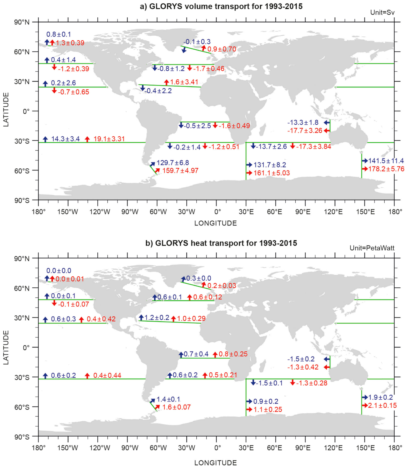
Figure 29. Mean 1993–2015 (a) volume (Sverdrup (SV = 10 6 m 3 /s)) and (b) heat (Petawatt (PW = 10 15 Watt) transports across the WOCE sections (green) from GLORYS reanalysis (see Section 1.6, endnote 13) (in red) with interannual standard deviation and Lumpkin and Speer’s (2007) estimations (in blue) with associated error. Arrows indicate the direction of the transport (positive in the northward and eastward directions).
