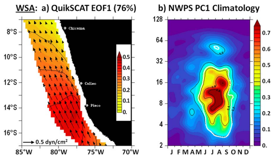
Figure 6. First mode of the bivariate EOF analysis of the subseasonal anomalies of the surface wind stress from QuikSCAT data: (a) Spatial pattern ( \text{dyn}/\text{cm}^2 ) showing wind stress vectors (arrows) and wind stress magnitude (color shading). (b) A 8 year climatology of the NWPS for the wind stress PC1 (PC1-WSA) estimated over the period June 2000 to May 2008. White line shows the 95% confidence level.
