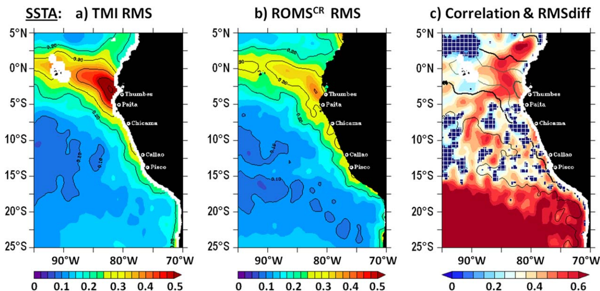
Figure A5. Analysis of daily Sea Surface Temperature intraseasonal (40–90 days) Anomalies (SSTA) over the 2000–2008 period: Map of variability (RMS) for (a) TMI-OI data and (b) ROMS CR simulation. (c) Map of correlation (color shading) and RMS differences (contours) between observed and simulated SSTA. Blue square patterns denote non-significant correlations (95% confidence level [Sciremammano, 1979]). Unit is °C.
