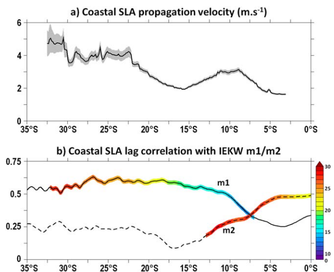
Figure 3. (top) Propagation velocity of the 0.5° coastal band averaged Sea Level intraseasonal Anomalies (SLA). At each latitude, the maximum lagged correlation between the coastal SLA at that latitude and the coastal SLA within a centered 7° latitudinal window is computed. For each 7°-window, the linear regression coefficient that best fit the lag estimation is calculated. Shading indicated error in the linear regression coefficient estimation. Unit is m s^{-1} . (bottom) Maximum lagged correlation between coastal (0.5° coastal band averaged) SLA with the first (second) Intraseasonal Equatorial Kelvin Wave (IEKW) mode at 100°W as a function of latitude in plain (dashed) line. Lag (in days) is specified with color shading. Positive value indicates that equatorial variability leads.
