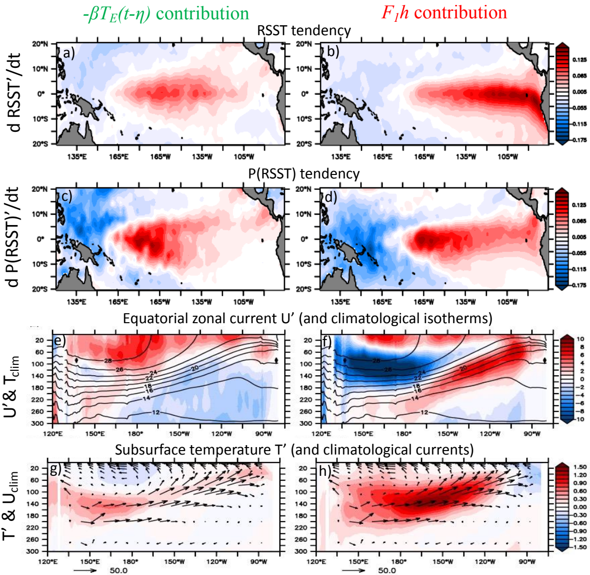
381 Fig. 2. Distinct physical processes represented by -\beta T_E(t-\eta) and F_I h terms in RDO, and related ENSO 382 spatiotemporal diversity captured by the RDO. a and b) contributions of respectively -\beta(x,y)T_E(t-\eta) and 383 F_I(x,y)h(t) to \partial T(x,y,t)/\partial t(t) in Equation 8.1 (i.e. the regression coefficients \beta(x,y) and F_I(x,y) for normalized 384 T_E and h , i.e. unit in ^{\circ}\text{C}\cdot\text{month}^{-1} per STD of T_E or h ) for obs2. By reconstructing T(x,y,t) from these patterns, 385 the RDO can simulate part of ENSO spatial and spectral diversity (cf. section 4f). c and d) as a and b, but 386 for the expected response of deep convection/precipitation to RSST tendency shown in a and b ( \text{mm day}^{-1}
