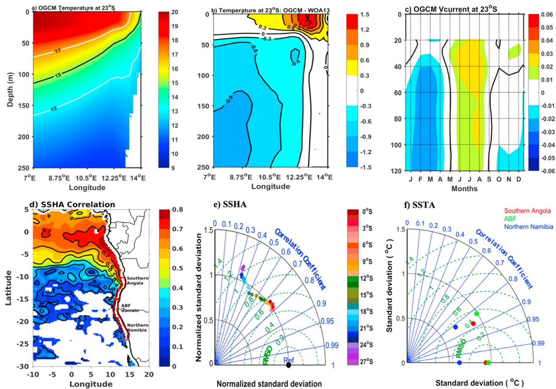
Figure 2. (a) OGCM mean (1958–2015) vertical temperature ( ^{\circ}\text{C} ) cross-shore section at 23^{\circ}\text{S} as a function of longitude and depth (m). The black (white) lines represent the mean position of the 15^{\circ}\text{C} ( 17^{\circ}\text{C} and 13^{\circ}\text{C} ) isotherms. (b) Difference between OGCM and observed (WOA13v2) mean vertical temperature ( ^{\circ}\text{C} ) section at 23^{\circ}\text{S} , with contours every 0.3^{\circ}\text{C} . (c) OGCM vertical profile of climatological meridional current velocities (m/s) at ( 14^{\circ}\text{E} , 23^{\circ}\text{S} ) to be compared to the ADCP climatology presented in Junker et al. (2017), their Figure 6a). The monthly mean climatology is computed over the 2003–2015 period. Positive (negative) current velocity values mean northward (southward) directed currents. (d) Correlation map between observed monthly detrended interannual AVISO SSHA and OGCM SSHA over the 1993–2015 period in the southeastern Atlantic Ocean. The white area depicts correlations nonstatistically significant at 95% (Sciremammano, 1979). Contours are every 0.1. Red contours highlight the positions of the three coastal domains of interest (see section 2.3.4). (e) Taylor diagram illustrating the OGCM skills in representing the altimetric detrended normalized SSHA along the southwestern African coast (averaged within the 1^{\circ} -width coastal fringe) over 1993–2015. Colors indicate the latitude. To subtract the mesoscale variability, time series are preliminarily smoothed using a 5^{\circ} -width latitudinal running average filter. (f) Taylor diagram comparing the OGCM and OI-SST detrended SSTA averaged within the three coastal (averaged within the 1^{\circ} -width coastal fringe) domains of interest (section 2.3.4), namely, Southern Angola ( 10^{\circ} – 15^{\circ}\text{S} ), ABF domain ( 15^{\circ}\text{S} – 19^{\circ}\text{S} ), and Northern Namibia ( 19^{\circ}\text{S} – 24^{\circ}\text{S} ) over the 1982–2015 period. Colored dots on the x axis represent the observations (OI-SST) in each domain.
