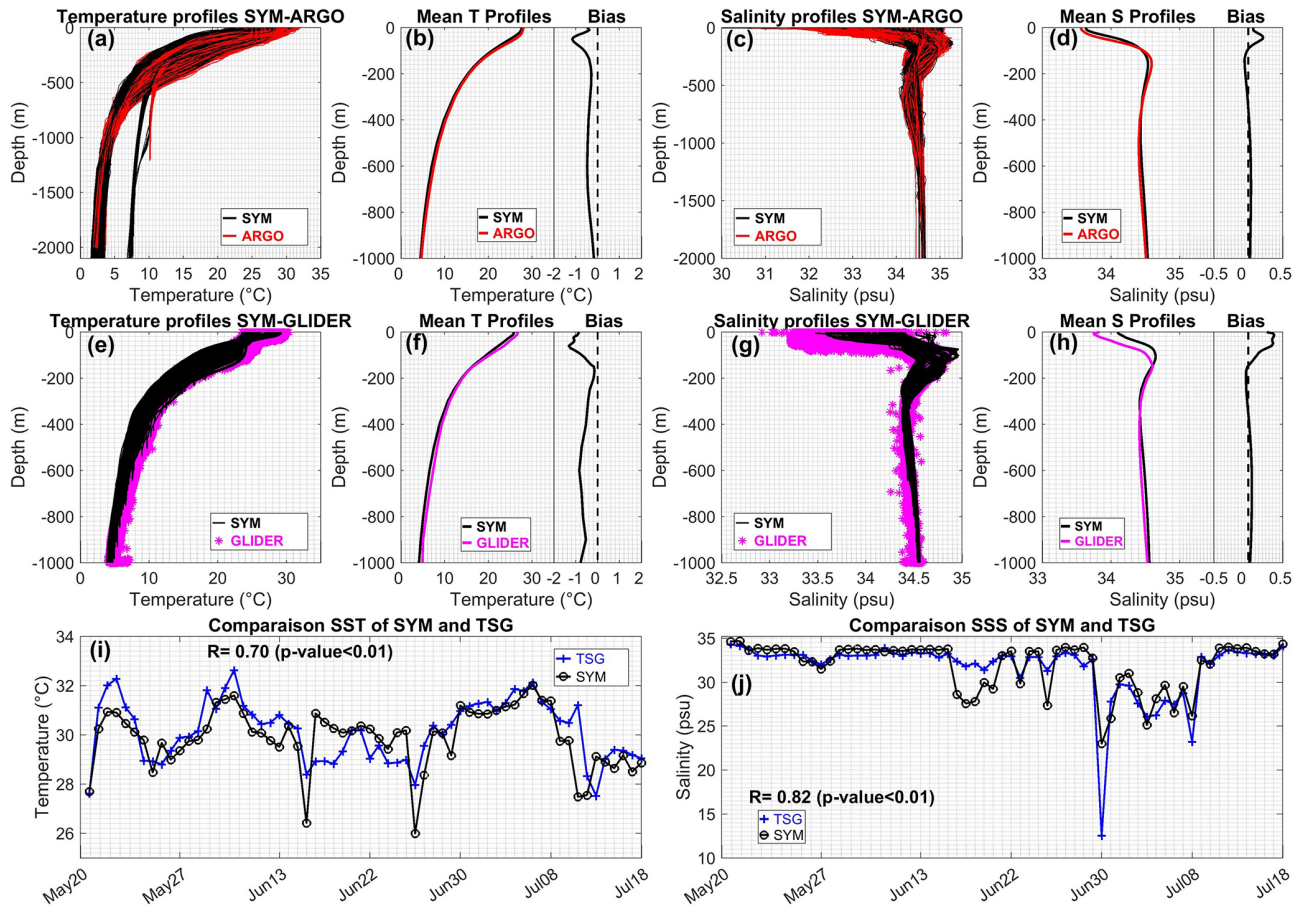
Figure 8. Temperature (°C) and salinity (psu) vertical profiles (all profiles, mean profiles, and mean bias between model and observations) from SYM4 outputs (black) compared with Argo floats (a, b, c, d, red) and glider measurements (e, f, g, h, magenta). (i) SST (°C) and (j) SSS (psu) from SYM4 (black) and TSG-Alis data (blue).
