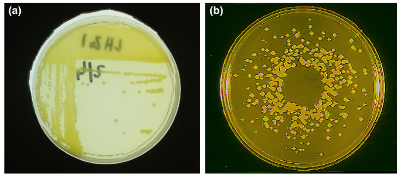
FIGURE 9 Typical colony morphology of Xanthomonas citri pv. citri on (a) YPGA medium and (b) KC medium after incubation at 28°C for 3 days. Photo courtesy: C. Vernière & O. Pruvost (CIRAD, FR).
