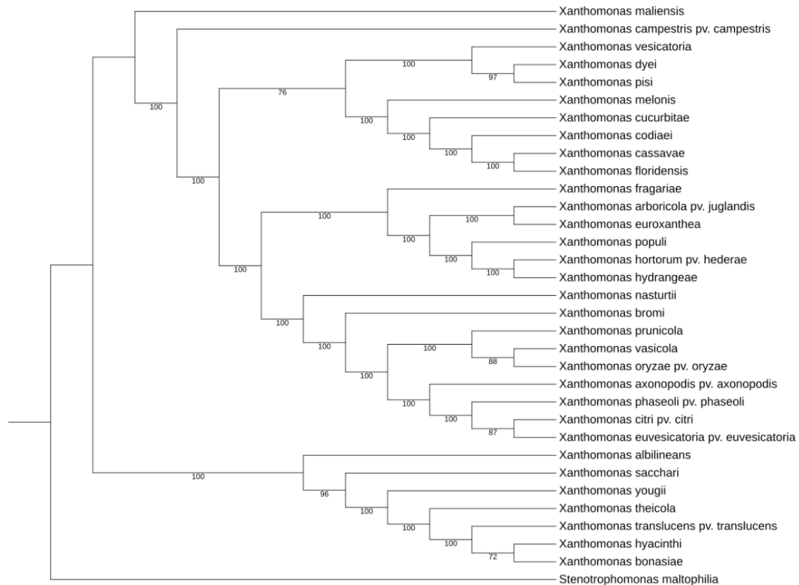
Figure 2 – Phylogenetic tree of the 32 valid species of Xanthomonas provided after TYGS analysis (Meier-Kolthoff et al., 2022). Tree inferred with FastME 2.1.6.1 (Lefort et al., 2015) from GBDP distances calculated from genome sequences retrieved from Genbank. The branch lengths are scaled in terms of GBDP distance formula d5. The numbers on branches are GBDP pseudo-bootstrap support values > 70% from 100 replications, with an average branch support of 97.2% (Farris, 1972). The Newick file was edited in iTOL ( https://itol.embl.de/ ) and rooted on the outgroup Stenotrophomonas maltophilia . The complete list of genomes and GenBank Assembly accession numbers are available in Supplementary Table S2.
