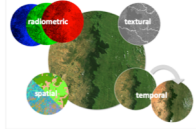
Fig. 2: Four types of features (spatial, radiometric, temporal and textural) can be extracted from remote sensing data.
