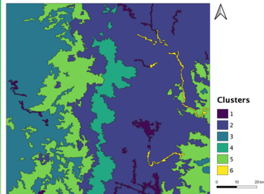
Fig. 4: Mapping of landscape units based on MODIS and Sentinel-2 data obtained with the combination of MODIS NDVI PCA between 2016 and 2020 and two texture methods (Haralick and FOTOTEX) applied on NDVI of Sentinel-2 data, in 6 clusters at two different dates: March and November in 2019. Haralick's Correlation and Entropy are the two indices used for the first method (Haralick).
