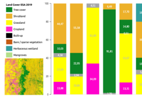
Fig. 6: Land cover distribution (ESA WorldCover 2019) map at 10 m spatial resolution in each cluster. The gray class represent the total of land cover classes showing less than 5% of the cluster area.
