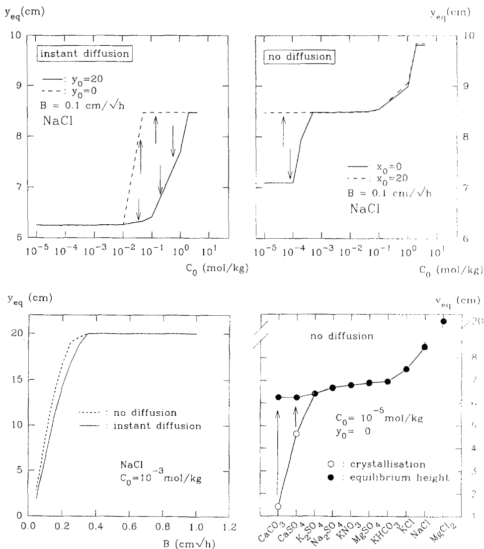
Figure 6 Evolution of equilibrium height taking into account the presence of salt.
