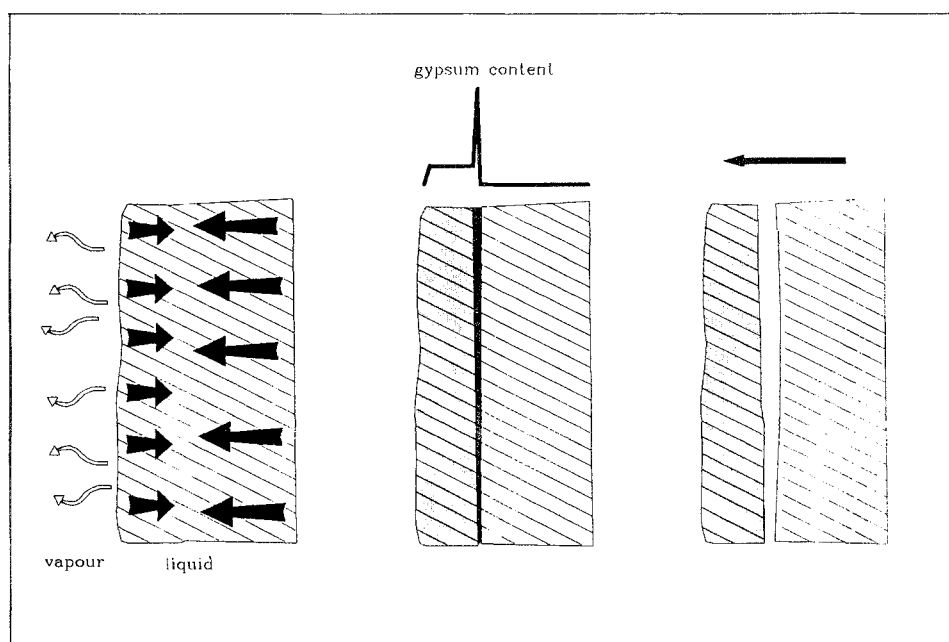
Figure 8 Schematic representation of the formation of contour scaling.
