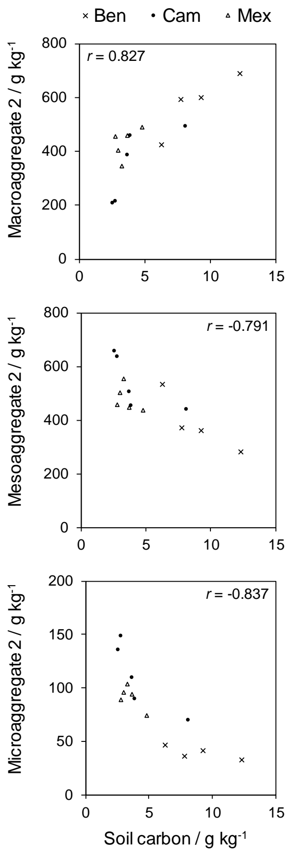
Figure 1 Relations between water-stable aggregation and carbon content in the 0-10 cm soil layer (Macroaggregate 2 >0.2 mm, 0.02< Mesoaggregate 2 <0.2 mm, Microaggregate 2 <0.02 mm, in g kg -1 soil <0.2 mm).
