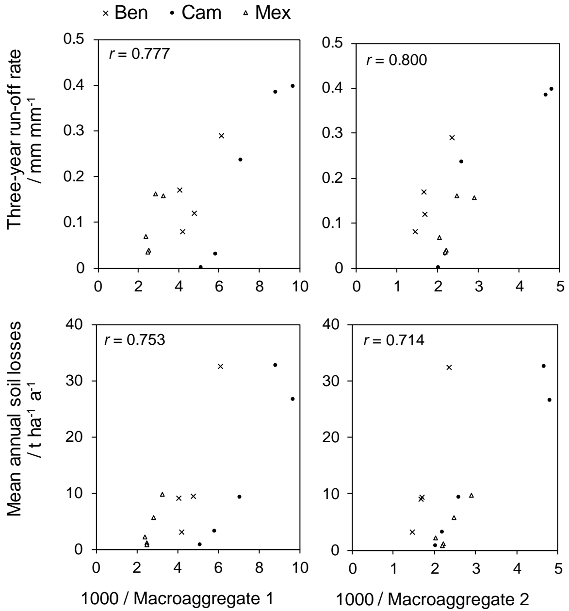
Figure 2 Relations between three-year run-off rate or mean annual soil losses and macroaggregate (>0.2 mm) content in the 0-10 cm soil layer (Macroaggregate 1 in \text{g kg}^{-1} soil <2 mm, Macroaggregate 2 in \text{g kg}^{-1} soil <0.2 mm).
