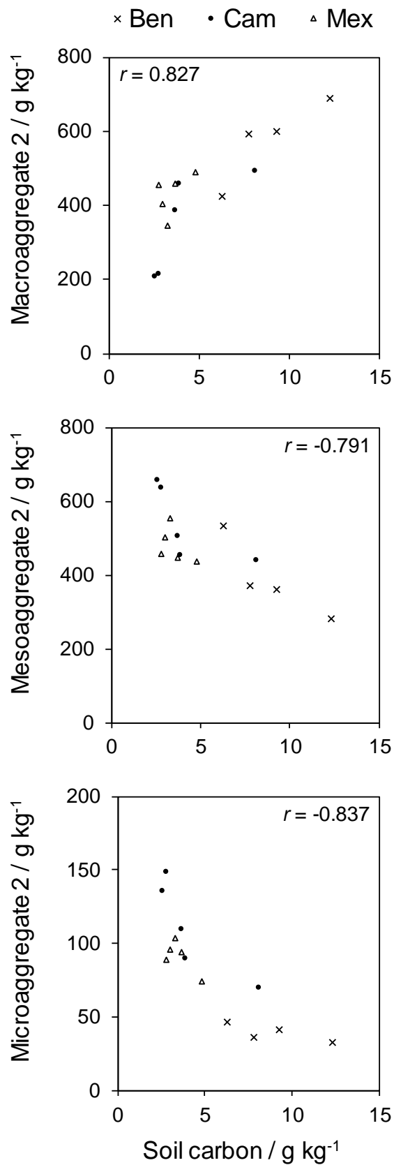
Figure 1 Relations between water-stable aggregation and carbon content in the 0-10 cm soil layer (Macroaggregate 2 >0.2 mm, 0.02 < Mesoaggregate 2 <0.2 mm, Microaggregate 2 <0.02 mm, in g kg -1 soil <0.2 mm).
