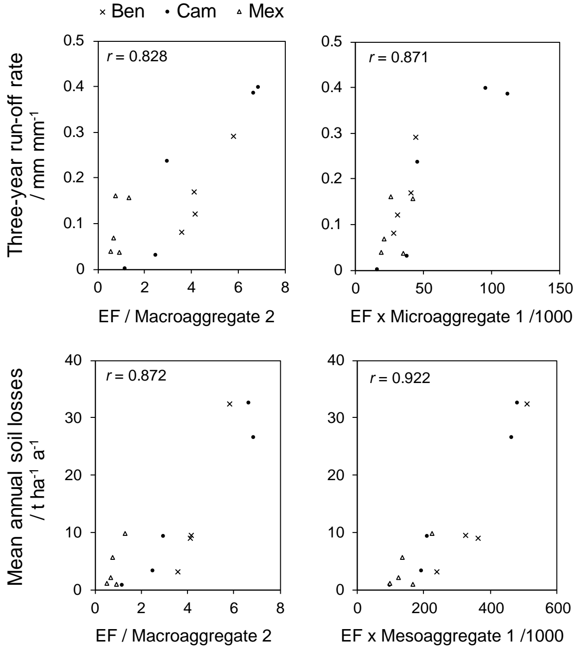
Figure 3 Relations between three-year run-off rate or mean annual soil losses, and Environment Factor (EF = mean rainfall erosion index \times slope gradient) and water-stable aggregation in the 0-10 cm soil layer (0.02 < Mesoaggregate 1 < 0.2 mm, Microaggregate 1 < 0.02 mm, in g kg -1 soil < 2 mm; Macroaggregate 2 > 0.2 mm, in g kg -1 soil < 0.2 mm).
