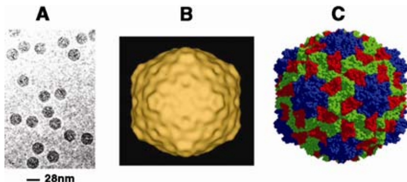
Fig. 4. Structure of Rice yellow mottle virus (RYMV) at different resolutions. A, Electron micrograph of frozen-hybridized native RYMV (Cryo-electron microscopy). B, Three-dimensional surface shaded density maps of RYMV derived by cryo-EM (49). C, Space-filling model of RYMV generated from X-ray crystallography data (54).
