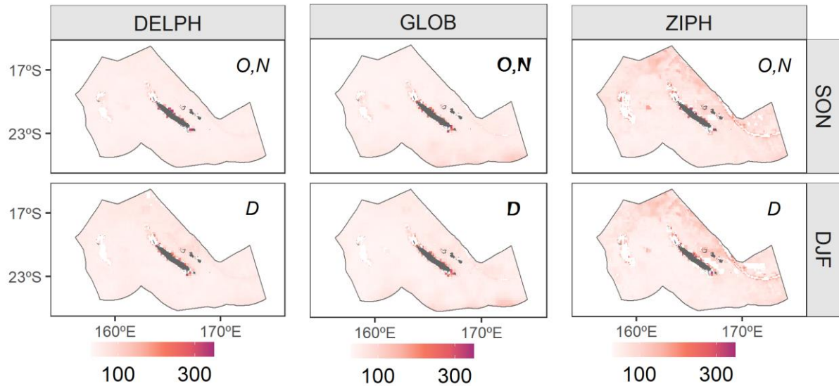
Supplementary Figure S7. Spatial predictions of standard error (expressed in %) for counts of individuals (of Delphininae (DELPH), Globicephalinae (GLOB) and Ziphiidae (ZIPH), by quarter in the New Caledonian EEZ. DJF: December, January and February; MAM: March, April and May; JJA: June, July and August; SON: September, October and November. Land is represented in grey. Reef and island names are indicated on Figure 1A . Areas in white include areas where no extrapolation was made and waters with bathymetry shallower than 300 m (identified on Figure 1 ).
