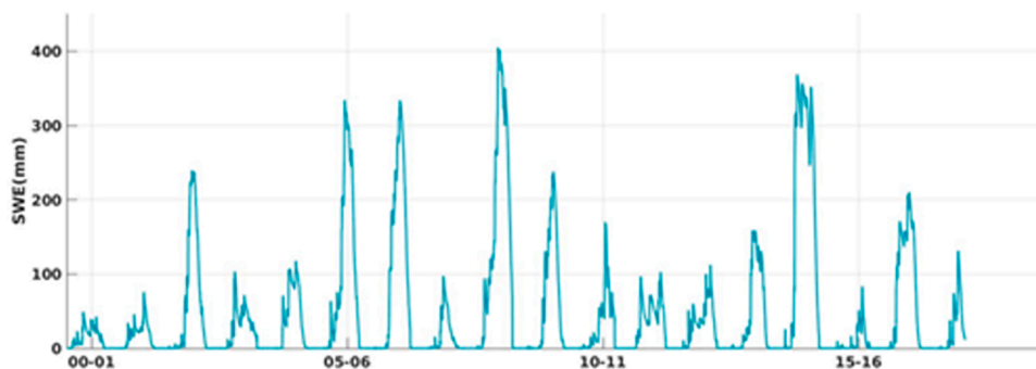
Fig. 11. Mean modeled snow water equivalent (SWE) over the Ourika catchment from 2000 to 2018.
