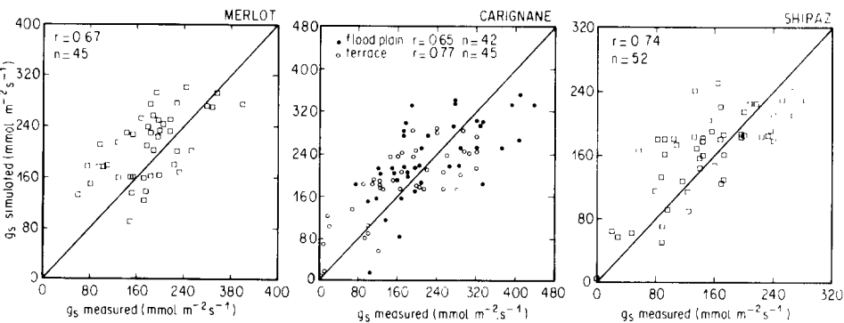
Fig. 3. Relationship between measured and simulated values of stomatal conductance ( r is the coefficient of correlation, n is the number of points).
