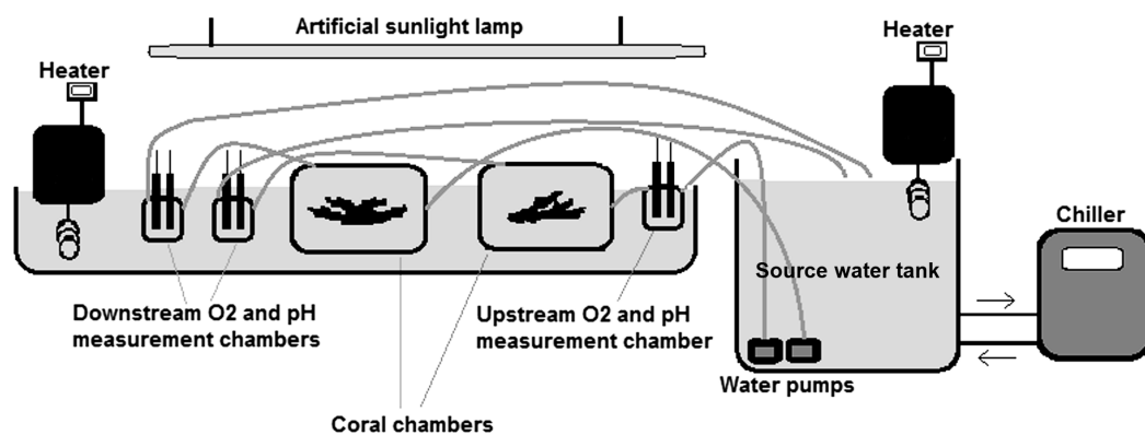
Figure 1 The experimental set up. Seawater collected from the study site was pumped from the source-water tank through the system at a constant rate of about 0.5 \text{ l. min}^{-1} . Oxygen concentration ( \text{mg. l}^{-1} ) and pH were recorded upstream and downstream the coral chambers every 5 min. 6,500 \text{ lux} light (i.e. about 120 \mu \text{ mol. m}^{-2} \cdot \text{s}^{-1} ) was provided by an artificial sunlight lamp (Dymax Rex-2). Water temperature was controlled by heaters (Lauda E100, with accuracy of \pm 0.1 \text{ }^\circ\text{C} ) and a chiller (Aqua medic Titan 1500, with accuracy of \pm 0.5 \text{ }^\circ\text{C} ). Net photosynthesis or respiration rate of corals was calculated in light and dark conditions as the difference in \text{O}_2 concentration between the upstream and downstream chamber multiplied by the flow rate. The measured metabolic fluxes were not affected by gas exchange with the atmosphere since the measurement and sample chambers were in a closed circuit and water was exposed to air only in the source tank.
