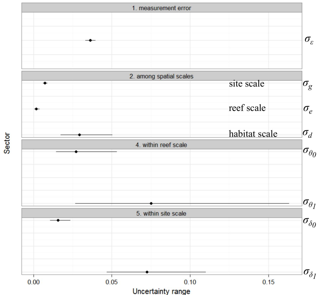
Figure 4. Estimation of the uncertainty in the three hierarchical stages of the model. The measurement error \sigma_{\epsilon} corresponds to the uncertainty at the data stage, and all other variance components \sigma account for uncertainty in the process model, decomposed into the variability in trend (intercept and slope) of coral cover at the three spatial scales of habitat, reefs and sites. doi:10.1371/journal.pone.0110968.g004
