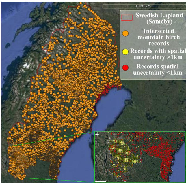
Fig. 2. Example of data visualization and balance between sampling effort (on field) of Birch tree GBIF dataset, its geographical uncertainties on the one hand and statistical needs for records and niche species modelling on the other hand. Note the systematic and squared sampling effort/strategy, in the southwestern part of the study area, presenting a significant spatial uncertainty (e.g. 2.5km, institution: ArtDataBanken). Nevertheless, this systematic sampling minimizes the bias due to presence-only data set, the species absence is noticeable in two areas. Even if overall autocorrelation (scale of the study area) might be over-represented, geographical information missed by an arbitrary cleaning constitutes a serious compromise to take into account in ecological modeling. Studied areas in Sweden: macro-regional scale (Swedish Lapland, Sameby), and micro-regional scale of analysis of Birch tree records from GBIF dataset (Sources: GBIF, Swedish Saami Parliament, RenGIS 2.0 sametinget.se; Lantmäteriet, SLU; realization R.Courault 2020)
