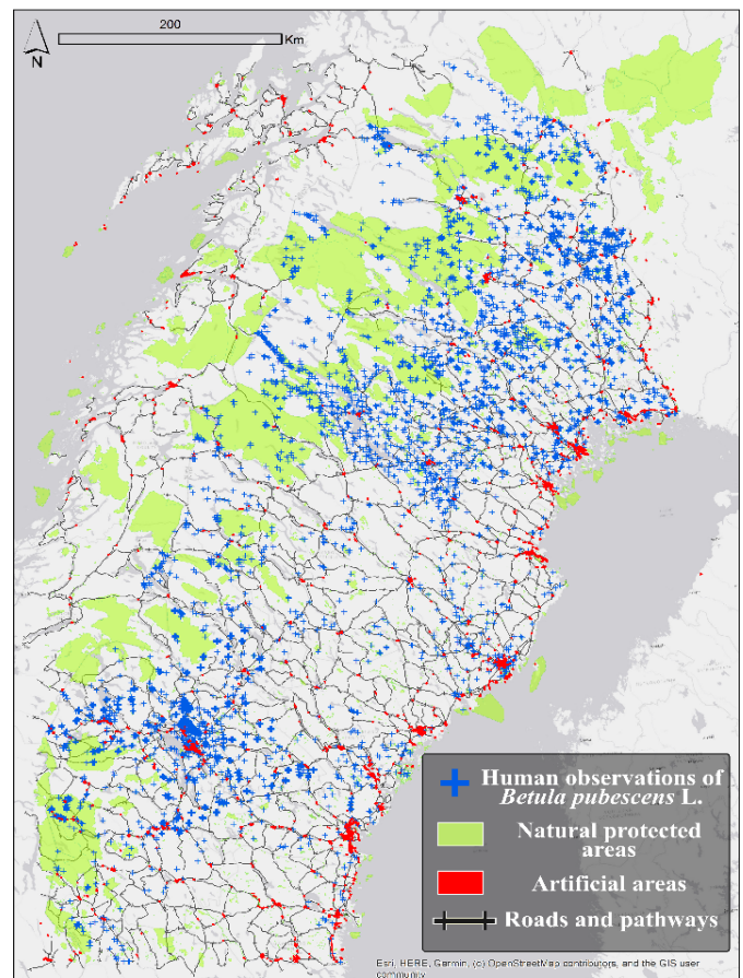
Fig. 3. Cartographic representation of filtered records of Birch tree and tested accessibility/facility factors (Sources: GBIF, Corine Land Cover 2018 Copernicus, European Environmental Agency and DivaGIS; realization R.Courault 2020)
