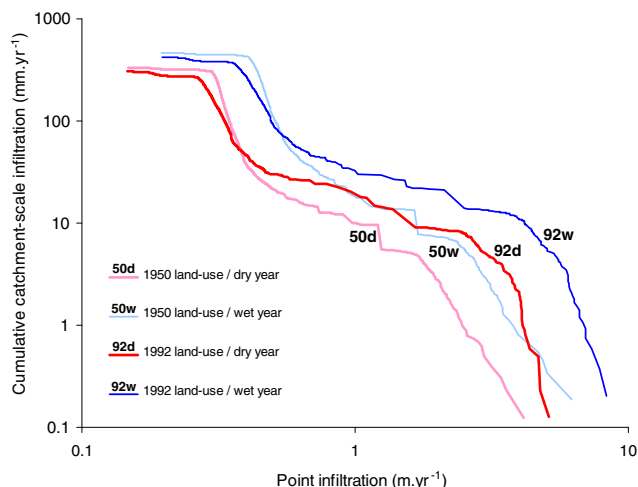
Fig. 11. Modelled point-to-catchment scale relationship for annual infiltration in Wankama catchment (pond excluded), before and after land use change. Each curve gives the catchment-scale flux (y-axis) infiltrated with point intensities above a given threshold (x-axis), for a given land use map (1950 or 1992) and rain season (dry or wet). Over the 42-year period, total catchment-scale infiltration decreased (top of curves), whereas concentrated infiltration (e.g., point rates greater than rainfall) increased spectacularly.
