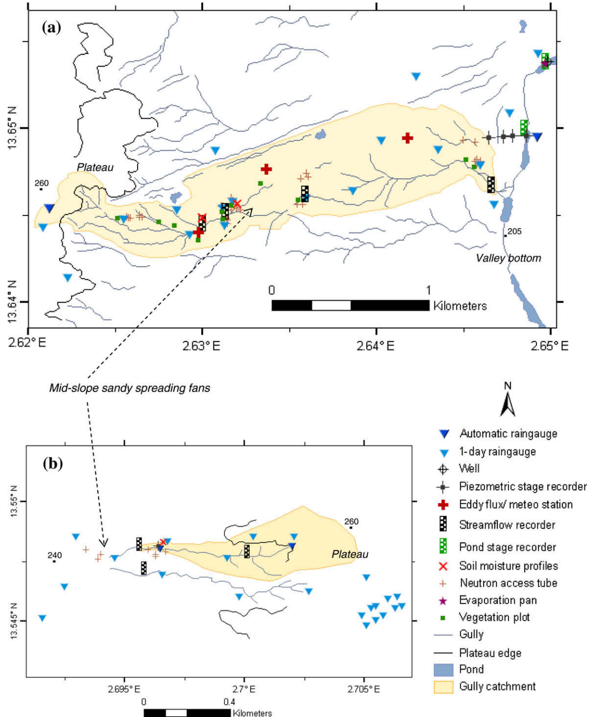
Fig. 9. Maps of Wankama (a) and Tondi Kiboro (b) local catchment sites.
