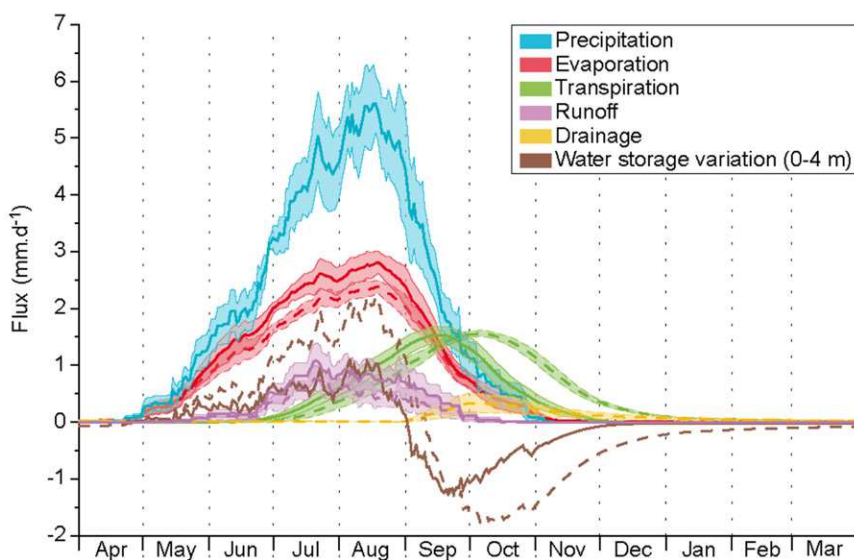
Fig. 8. Estimated mean seasonal courses of water cycle components for fallow (solid lines) and millet (dashed lines) plots: fluxes and rate of storage change in the 0- to 4-m soil column. Means are computed across years and for a 30-d running window. Light-colored intervals show a variation of \pm 1 standard estimation error (after Velluet et al., 2014).
