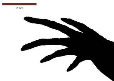
Celaticincus similis
