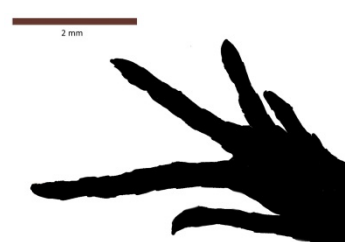
Graciliscincus shonae
