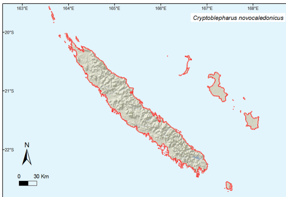
C. novocaledonicus
