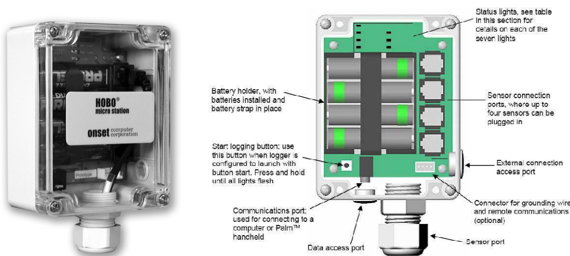
Figure 11 : Centrale d'acquisition
