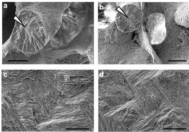
Figure 4. Microstructural comparison between modern and fossil (this study) corals and giant clam (SEM images, scale: 50 \mu\text{m} ). Massive coral Porites sp. specimens: (a) modern coral VA EPI; (b) early mid-Holocene coral Psp-07-09, with arrow indicating center of calcification. Giant clam Tridacna maxima specimens: (c) modern giant clam T-02-09; (d) early mid-Holocene giant clam T-10-09 (scale 50 \mu\text{m} ).
