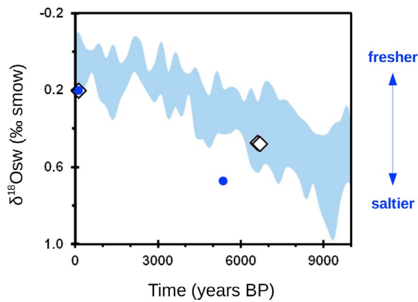
Figure 9. Holocene \delta^{18}\text{O}_{\text{sw}} evolution in the Western Pacific area – Diamond: coral data (this study), Blue dots: coral data from Gagan et al. [1998]. Blue area – foraminifer’s data from sediment cores ODP806B, MD70, MD76 and MD81. The blue area represents one standard deviation interval of the mean values calculated from the four sedimentary records [ Lea et al. , 2000; Stott et al. , 2004].
