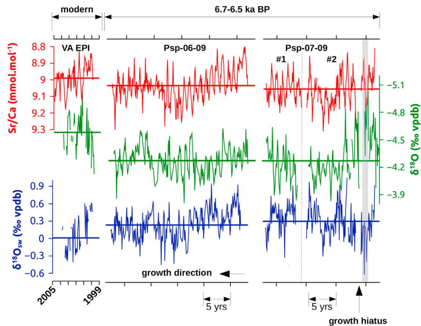
Figure 5. Monthly resolved geochemical data obtained from the modern and the two fossil Porites sp. corals from Vanuatu: Sr/Ca (red), \delta^{18}\text{O} (green) and \delta^{18}\text{O}_{\text{sw}} (blue). The thick horizontal line represents the average value of each record. The growth hiatus of the colony Psp-07-09 is showed by the black arrow and the shaded area indicates the anomalous part of the record not included in the study (cf. text). Note that both Sr/Ca-axis and \delta^{18}\text{O} -axis are inverted.
