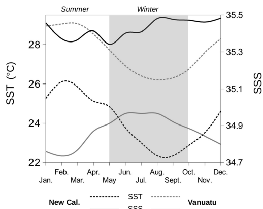
Figure 3. Instrumental SST and SSS data. The modern SST and SSS conditions in New Caledonia were recorded by a thermo-salinograph located on the Fausse Passe de Uitoé reef (22.28°S, 166.98°E), from 1992 to 2009. Data were provided by the Réseau d'observation des stations côtières of the Institut de Recherche pour Développement (IRD-Nouméa, New Caledonia). Vanuatu SSS data for the 1949 to 2008 period came from a 2^{\circ} \times 2^{\circ} grid, centered on 16°S, 165.5°E [Gouriou and Delcroix, 2002]. SST data was selected for the period 1970–2011 on a 3^{\circ} \times 3^{\circ} grid, centered on 15.5°S, 164.5°E (HadISST1.1) [Rayner et al., 2003].
