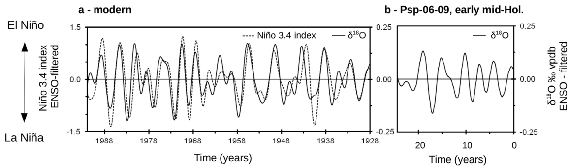
Figure 8. Comparison of modern versus early mid-Holocene ENSO amplitudes. (a) ENSO-filtered modern coral \delta^{18}\text{O} data [data from Kilbourne et al. , 2004] and El Niño 3.4 Index. (b) Porites sp. Psp-06-09 ENSO-filtered \delta^{18}\text{O} data.
