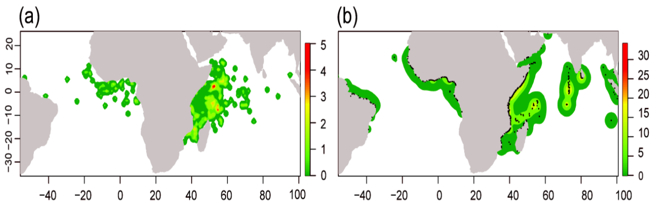
Figure 19. Smoothed densities of DFAD deployment positions (a) and related beaching events (b); black dots correspond to individual beaching positions (Maufroy et al. 2015)
