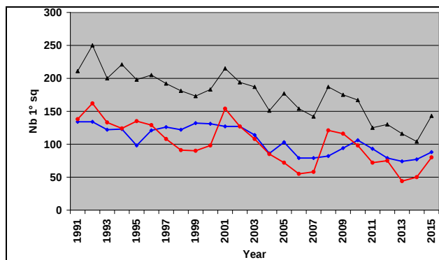
Figure 15. Yearly numbers of 1° with YFT catch >20 t, on Free schools sets.
