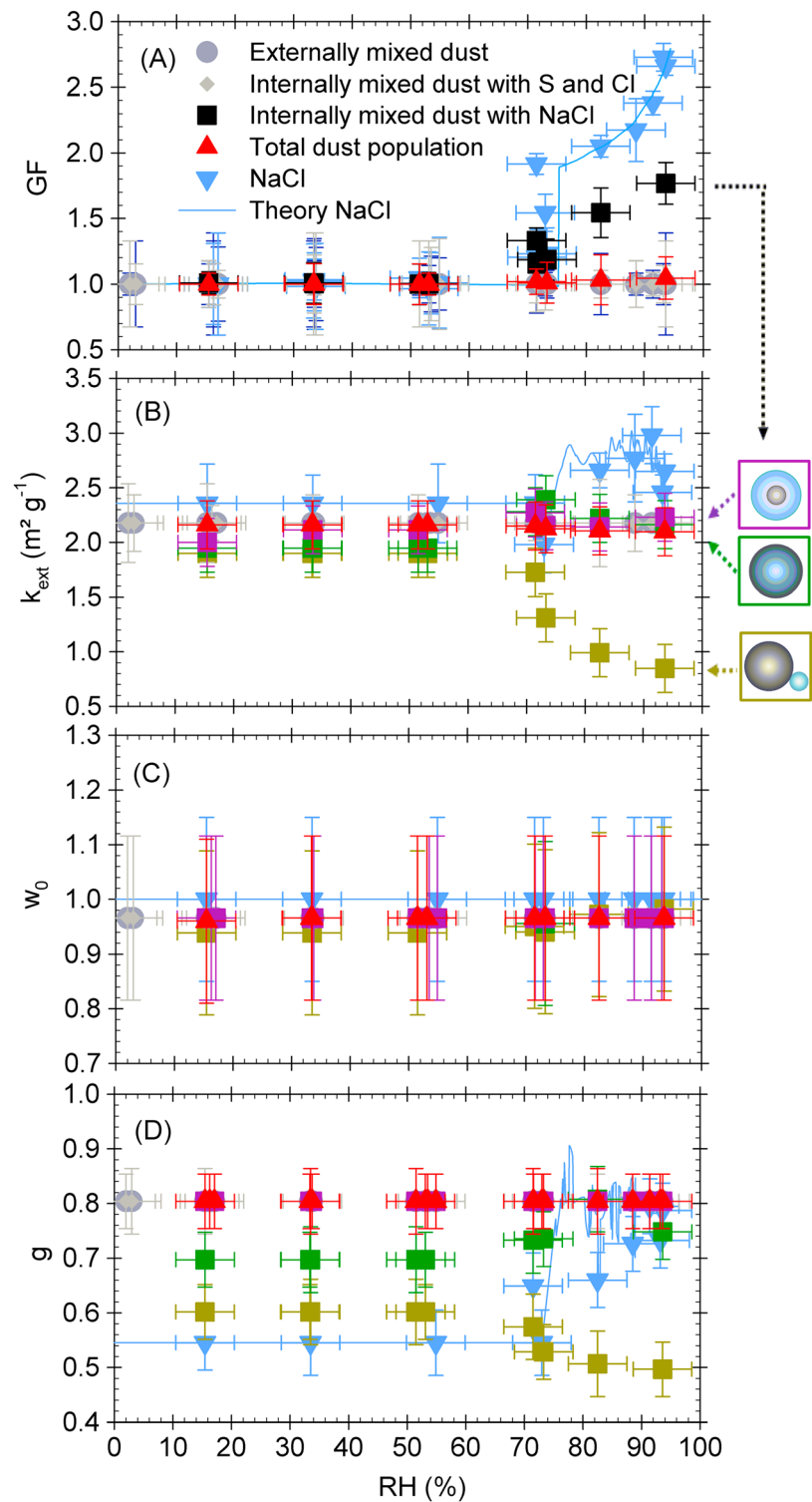
Figure 3. (a) Hygroscopic growth factor (GF), (b) scattering mass efficiency ( k_{ext} ), (c) single-scattering albedo ( w_0 ), and (d) asymmetry parameter ( g ) at \lambda = 550 nm as a function of relative humidity for each particles type. Externally mixed dust particles, i.e., S, Cl, and Na, were not detected and are shown in dark grey circles, dust internally mixed with sulfate or chloride in grey diamonds, and relatively pure NaCl particles in blue triangles. Dust aggregated with NaCl particles is shown in black squares in Figure 3a and is separated for the different dust mixing state with NaCl in Figure 3b, with green squares representing the homogeneous mixing, purple squares for the core-shell mixing, and golden squares for the aggregate structure. GF and k_{ext} of the total dust population (red triangles) were calculated using GF and k_{ext} values of single dust particles and the contribution of each particle type.
