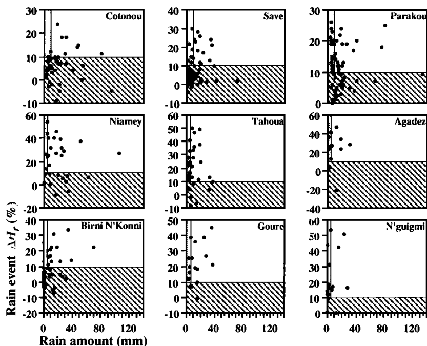
Figure 6. Relative humidity variation versus rainfall amount for nine stations. In the shaded left-hand rectangles limited by \Delta H_r = 10\% , dots correspond to rains with high variations of relative humidity and small amounts. In the lower hatched rectangles, dots correspond to rains with small variations of relative humidity for any rainfall amount.
