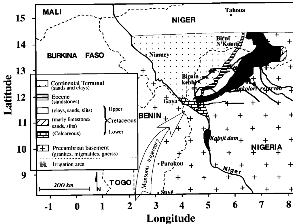
Figure 7. Regional geology and surface water management near Birmi N'Konni. Air masses from the south may be recharged over the Kainji dam, the Bakolori reservoir, and the irrigated areas.
