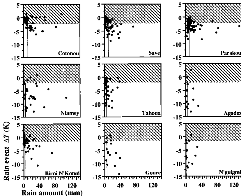
Figure 5. Variation of temperature \Delta T versus rainfall amount for nine stations. In the upper hatched rectangles limited below by \Delta T = -2 K, dots correspond to rains with low temperature variations for any rain amount. In the shaded left-hand rectangles, dots correspond to rains with small amounts and large temperature decreases.
