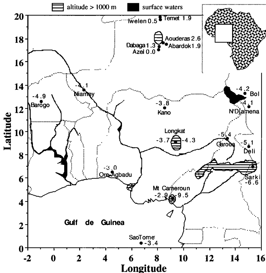
Figure 1. Location of stations where isotopic rainfall data were published in the region. Horizontal axis shows longitude in degrees. Vertical axis shows latitude in degrees north. Numbers are the weighted mean values of \delta^{18}O in per mil at observation stations. For Longkat and Mount Cameroon each value corresponds to a different station at a different altitude (Table 1).
