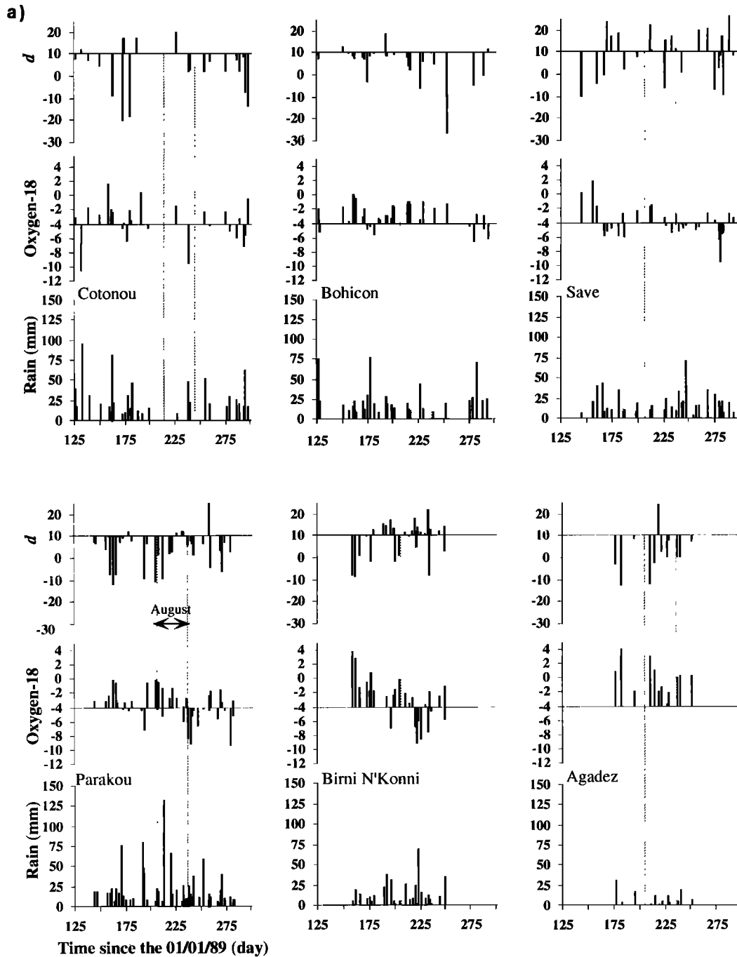
Figure 4. Rainfall event data from 1989, including rain amount, oxygen-18 and d versus time. (a) Stations from south (Cotonou) to north (Agadez). (b) Stations from west (Niamey) to east (N'guigmi) in the Sahelian zone.
