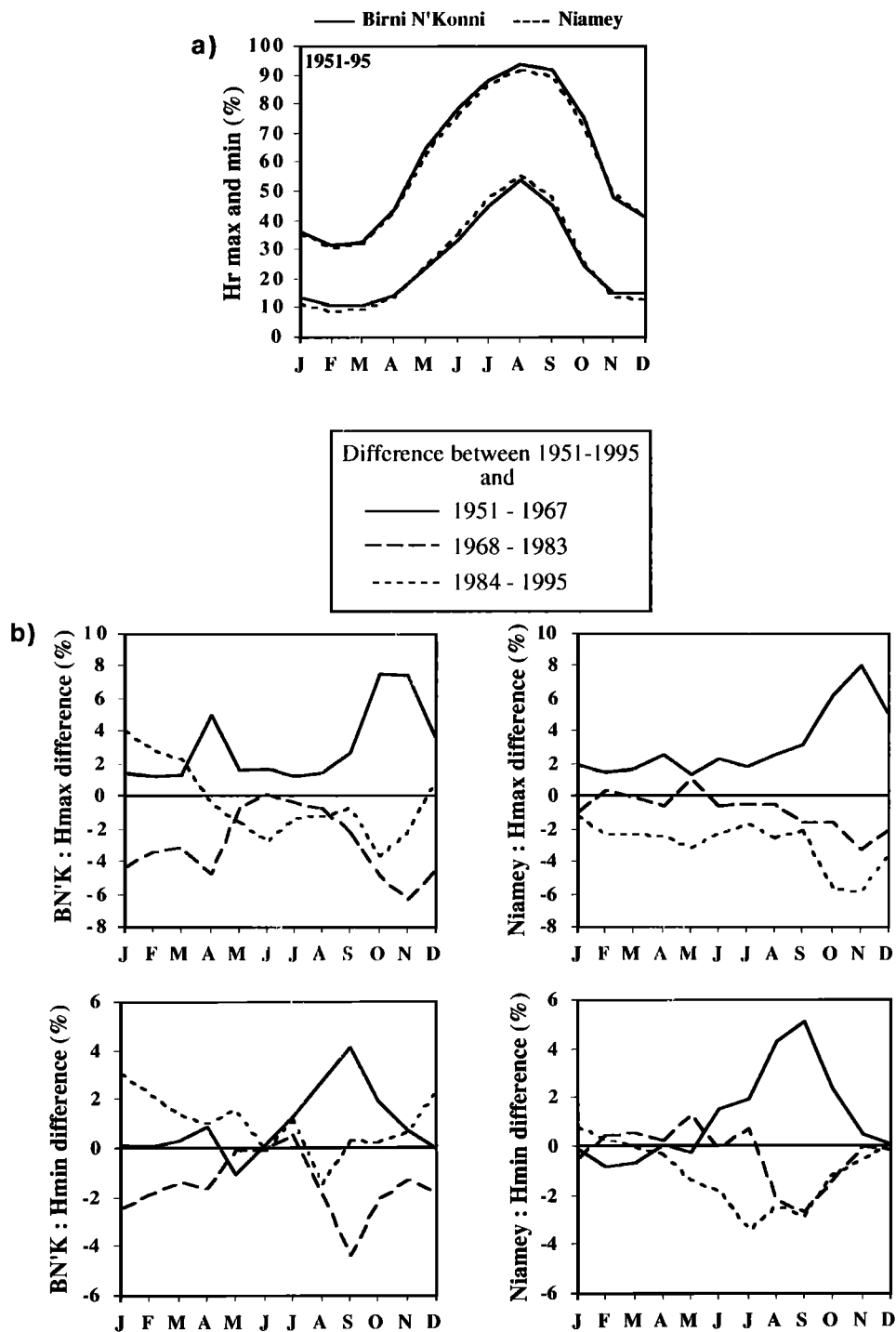
Figure 8. Relative humidity in Niamey and Birni N'Konni (BN'K) from 1951 to 1995. (a) Year-to-year monthly mean of daily maximum and minimum relative humidity. Niamey and Birni N'Konni show almost the same evolution. (b) Difference between the mean values over the period of 1951-1995 and the mean values over other periods. The upper plots show the difference in maximum relative humidity, and the lower plots show the difference in minimum relative humidity. For the humid period of 1951-1967 the difference is mainly positive for both stations. For the dry period of 1968-1983, differences are negative. For the dry period of 1984-1995, differences are negative for Niamey but positive for Birni N'Konni during the dry season, which could be linked to the irrigation in the Sokoto valley.
