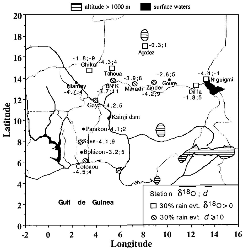
Figure 2. Location of stations sampled during the 1989 rainy season (EPSAT program). Numbers are the weighted mean values in per mil of \delta^{18}\text{O} and deuterium excess for this period. Shaded squares are stations where more than 30% of rainfall events have \delta^{18}\text{O} > 0\text{‰} (numerous rainfall events affected by evaporation). Hatched circles are stations where more than 30% of rainfall events have a deuterium excess of more than 10‰ (contribution of vapor originating from evaporation over the continent).
