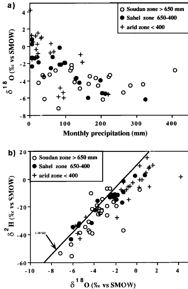
Figure 3. Monthly weighted mean values from rainfall event values from 1989: (a) \delta^{18}\text{O} versus rain amount and (b) \delta^2\text{H} versus \delta^{18}\text{O} . Sudanese zone includes Bohicon, Cotonou, Parakou, Save, and Gaya; Sahelian zone includes Birni N’Konni, Maradi, Niamey, and Zinder; and Arid zone includes Agadez, Chikal, Diffa, N’guigmi, Gouré, and Tahoua. SMOW, Standard mean ocean water.
