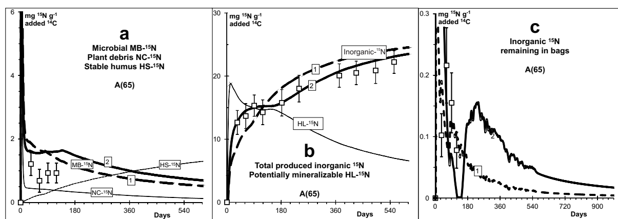
Fig. 3. Measured and simulated values at the lowest site (A65): squares are measured data with 95 % confidence intervals of (a) MB- ^{15}N , (b) total inorganic- ^{15}N , (c) inorganic ^{15}N remaining in bags; heavy dashed lines (1) are the simulated values using assumption 1 of constant C : N ratio of MB; heavy solid lines (2) are the simulated values using assumption 2 (variable C : N ratio of MB) and the first strategy (a); the light dotted line in (a) is the simulated ^{15}N in stable humus HS, the light dashed line in (a) is the ^{15}N remaining in the plant necromass (NC) and the light solid line in (b) is the potentially mineralizable ^{15}N in the labile humus HL.
