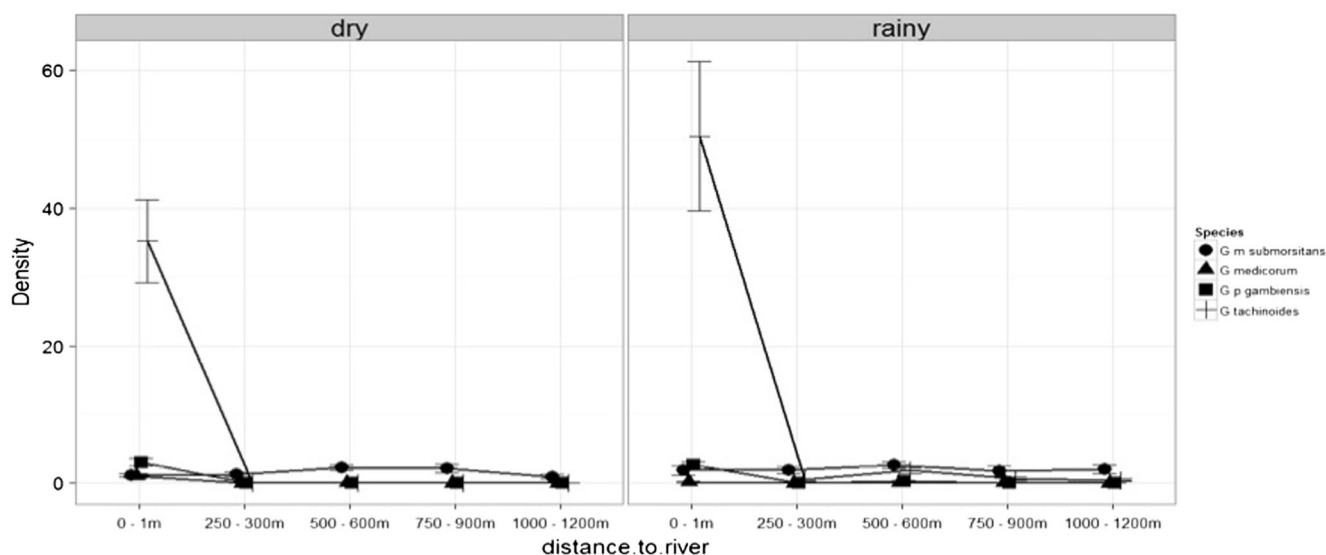
Fig. 2 Seasonal variation of tsetse densities depending on the distance to the river
