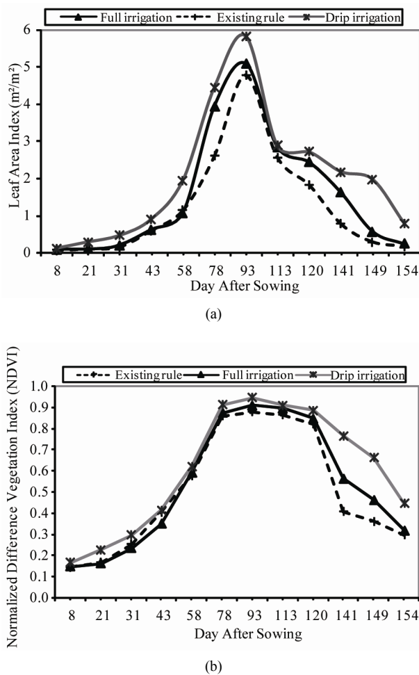
Figure 1. Seasonal time course of LAI and NDVI of winter wheat for the three irrigation treatments.
