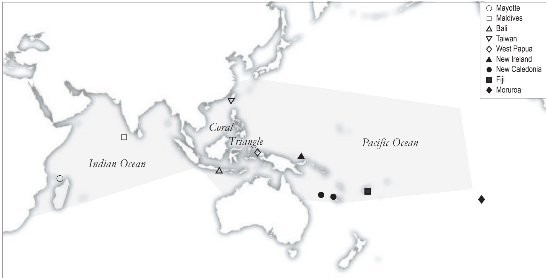
Fig. 2. Longface emperor, Lethrinus olivaceus . Sampling locations of individuals selected for morphometric analysis and/or genetics. Mayotte: Bancs Geysier and Z  lee, Mozambique Channel, April 2011 ( N=2 ); Maldives: Baa atoll, June 2008 ( N=4 ); Bali: Kedonganan fish market, February 2007 ( N=5 ); Taiwan: Kenting, May-June 2011 ( N=4 ); West Papua: Sorong, November 2007 ( N=6 ); New Ireland: Kavieng, August 2006 ( N=1 ); New Caledonia: Northern lagoon, April 2007 ( N=22 ) and Chesterfield Islands, Coral Sea, August 2011 ( N=1 ); Fiji: Tai Levu, September 2008 ( N=1 ); Moruroa: Moruroa lagoon, June 2006 ( N=8 ). Shaded: distribution of the species, as inferred from the point map provided by FISHBASE [10] (accessed 02 November 2012).
