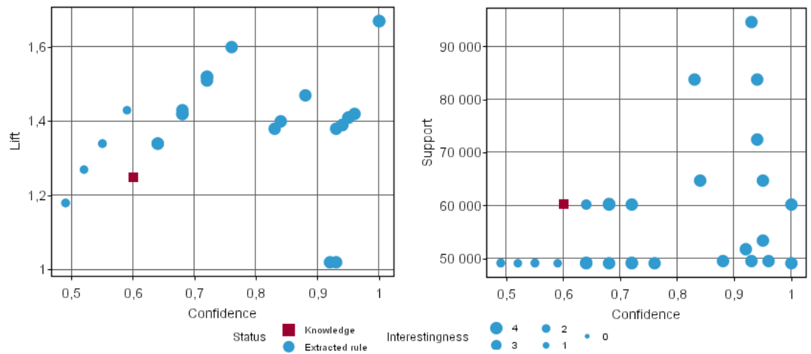
Figure 4: Extracted rules (dots) matching knowledge rule 565 (square) (IMAK interestingness value increase with dot size) a) Confidence vs Lift - b) Confidence vs Support
