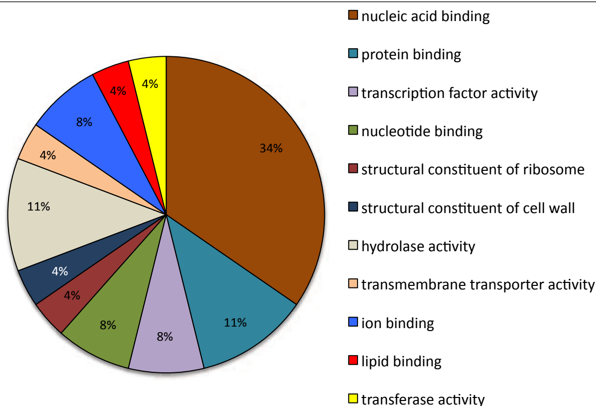
Figure 4 34 EST-SSRs that detect polymorphisms can be assigned Gene Ontology molecular function annotations. The graph depicts the level 3 molecular function annotations.
