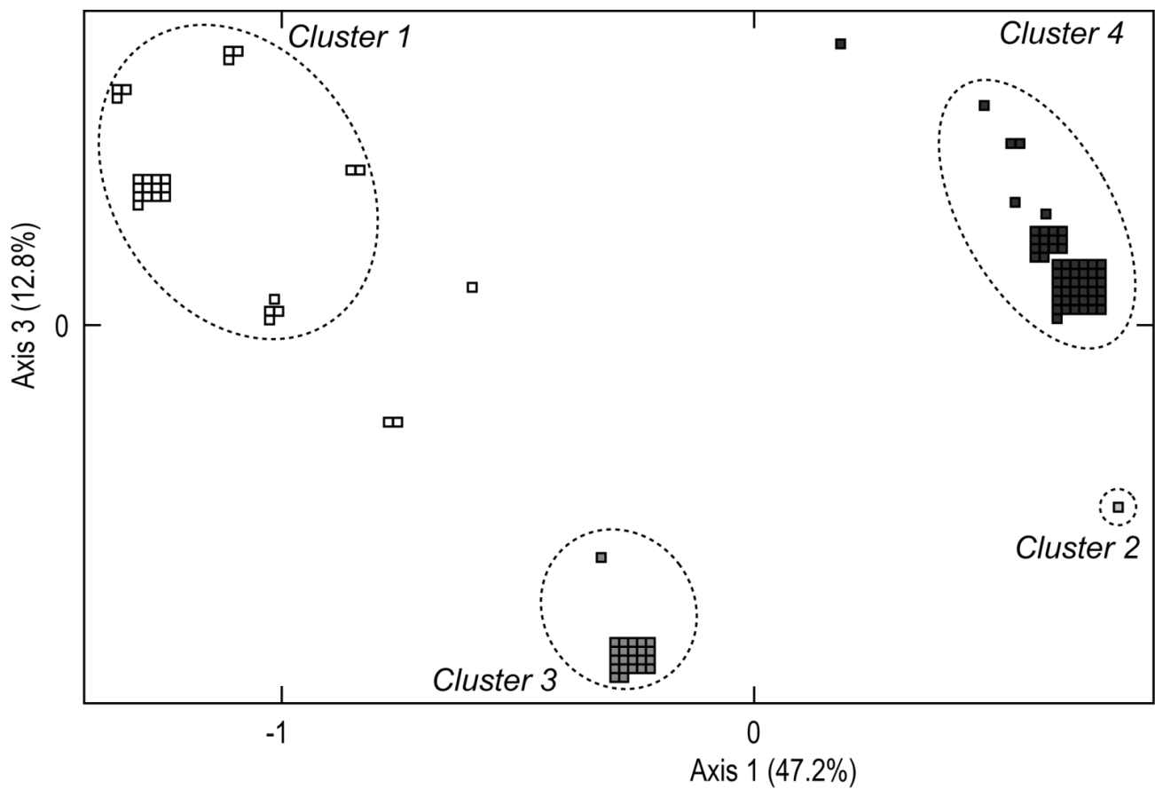
Fig. 1 Himantura uarnak species complex. Correspondence analysis (CA) (GENETIX: Belkhir et al. 2000) on individuals (squares) defined by their genotypes at five polymorphic intron loci. Ellipses delineate clusters of individuals with assignment >90% to either one of three clusters (1, 3, 4) obtained from Bayesian structure analysis (STRUCTURE: Falush et al., 2007). ‘Cluster 2’ corresponds to a single individual, which was singled out on Axis 2 of CA (not shown). Individuals geometrically intermediate between Cluster 1 and either Cluster 3 or Cluster 4 were interpreted as backcross offspring (see text and Appendix 1). Mitochondrial-DNA clade of each individual (see Fig. 2) is indicated by a distinct tone of grey: open , Clade I; light grey , Clade II; dark grey , Clade III; charcoal black , Clade IV.
