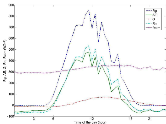
Fig. 2. Illustration of the typical course of AE, R_g , G , R_n and R_{atm} during a day (day 124, Auradé 2006).
