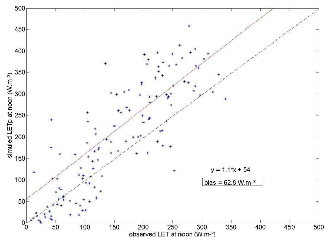
Fig. 5. Observed ET at noon compared with simulated ETP on unstressed days, example for Auradé 2006.
