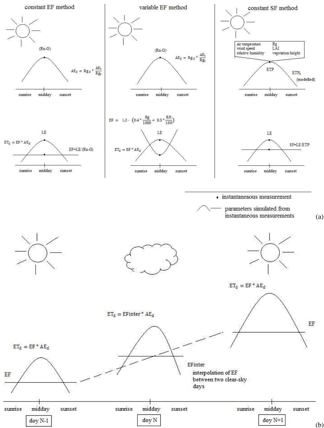
Fig. 1. Illustration of EF and SF methods to retrieve daily and seasonal ET. (a) Illustration of EF and SF methods to reconstruct daily ET from instantaneous measurements and (b) illustration of method to retrieve ET on cloudy days.
