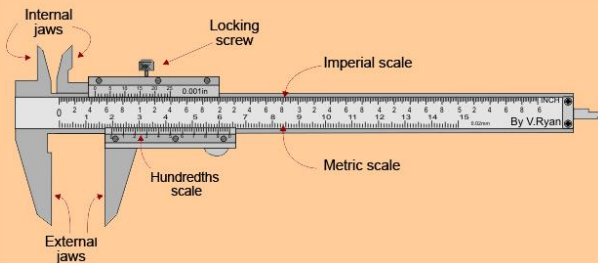
Figure 30: Drawing of a Vernier caliper
