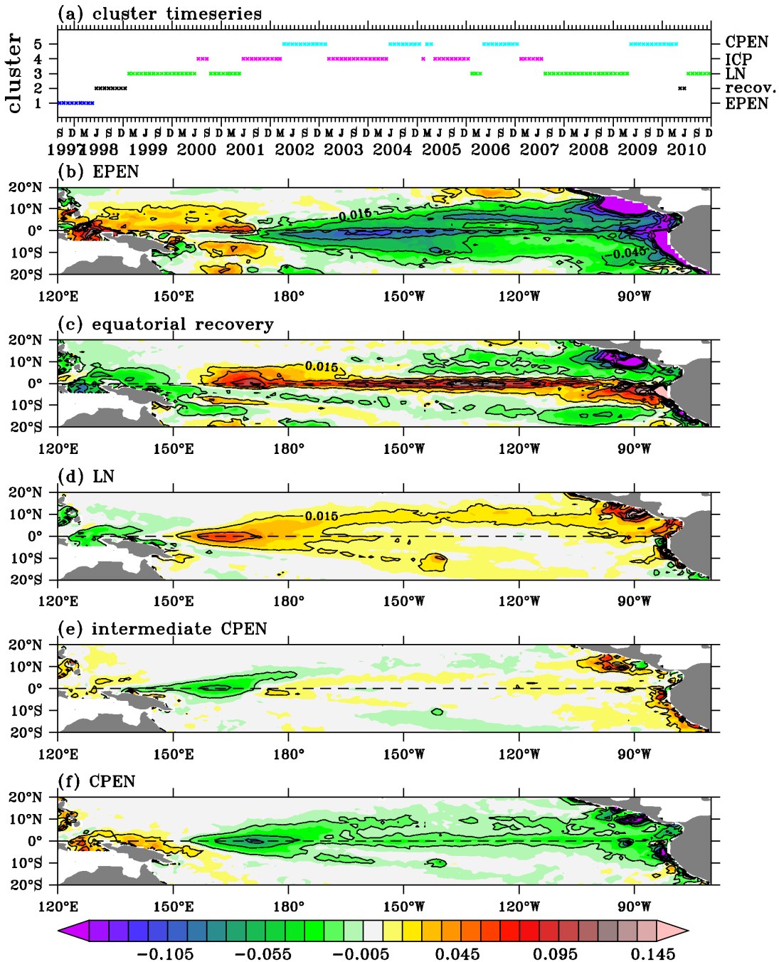
18 Figure 4. (a) Time series of the cluster analysis. Spatial patterns of the corresponding surface 19 chlorophyll anomaly during the so-called (b) Eastern Pacific El Niño (EPEN), (c) equatorial 20 recovery conditions (recov), (d) La Niña (LN), (e) intermediate Central Pacific period (ICP), 21 and (f) Central Pacific El Niño (CPEN). Chlorophyll anomaly contours are every 0.03 22 \text{mg m}^{-3} . The 0 \text{mg m}^{-3} contour is omitted.
