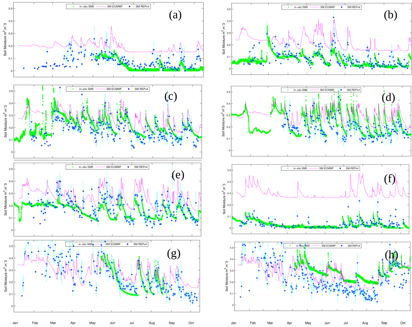
Fig. 6 Time series plots of soil moisture retrievals from SMOS vs SCAN site 2160 (a), 2018 (b), 2018 (c), 2018 (d), 2018 (e), 2018 (f), 2018 (g), 2018 (h).
