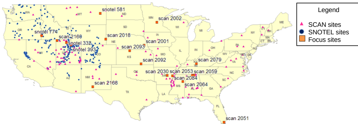
Fig. 4 Location of selected SCAN/SNOTEL sites
