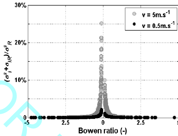
Figure 2 Contribution of absorption (\sigma_{IR}^2 + \sigma_I^2)/\sigma_R^2 estimated from theoretical equations versus the Bowen ratio for various wind speeds (0.5 and 5 m s -1 )
