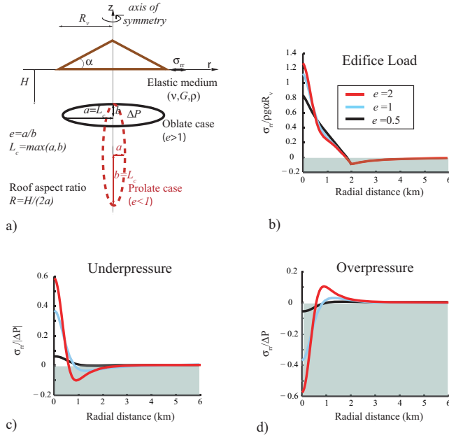
Figure 1. Model geometry and stress field induced at the Earth's surface. a) Model geometry and key parameters. b) Radial stress ( \sigma_{rr}(r) ) induced at the Earth's surface by an edifice load (radius R_v = 2 km) when the magma reservoir is at lithostatic equilibrium ( \Delta P = 0 ). The stress is normalised by the load applied at the axis. c) Radial stress ( \sigma_{rr}(r) ) induced at the Earth's surface by an underpressurized magma reservoir ( \Delta P < 0 ) with no edifice at the surface. The stress is normalised by the magma reservoir underpressure ( |\Delta P| ). d) Radial stress ( \sigma_{rr}(r) ) induced at the Earth's surface by an overpressurized magma reservoir ( \Delta P > 0 ) with no edifice at the surface. The stress is normalised by the magma reservoir overpressure ( \Delta P ). Radial stress calculations are obtained for a reservoir depth H of 0.5 km and maximum extension L_c of 0.5 km. Poisson's ratio is equal to 0.25. The black, blue and red curves are obtained, respectively, for a reservoir ellipticity ( e ) of 0.5, 1 and 2. The grey area corresponds to tensile stress (negative values).
