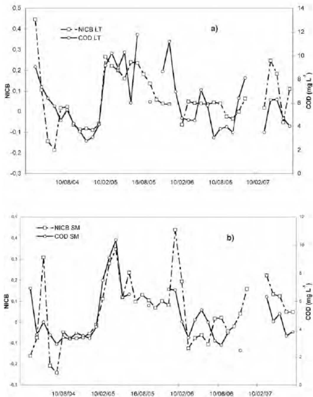
Fig. 5. NICB vs COD (mg L -1 ) content at Langa Tabiki (a) and Saut Maripa (b)
