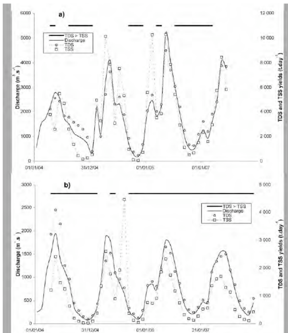
Fig. 3. Monthly discharge, dissolved and suspended sediment yields for (a) the Maroni River at Langa Tabiki (2004-2008 and (b) the Oyapock River at Saut Maripa (2004-2008). It should be noted that TDS is > to TSS nearly 95% of time for Oyapock and about 50% for Maroni.
