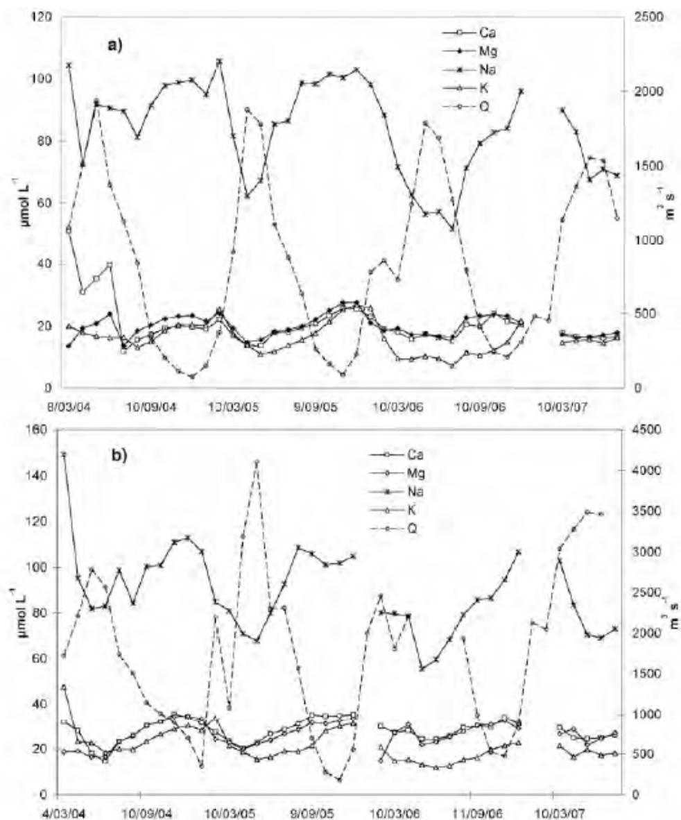
Fig. 6. Major cations content and water discharge at Saut Maripa (a) and Langa Tabiki (b)
