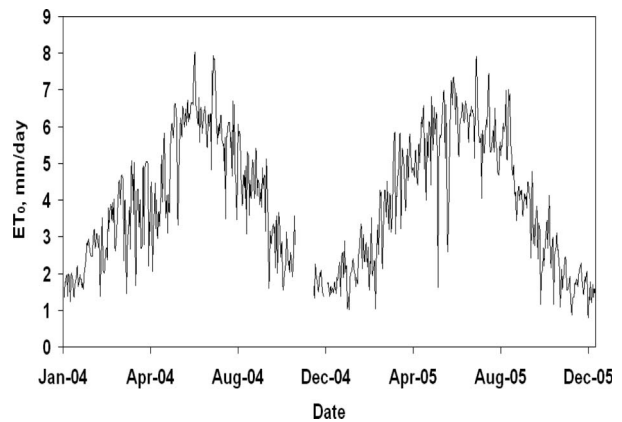
Figure 2. Daily reference evapotranspiration ET_0 calculated following the FAO-Penman-Monteith equation during the 2004 and 2005 growing seasons of citrus orchards in the Tensift Al Haouz basin.
