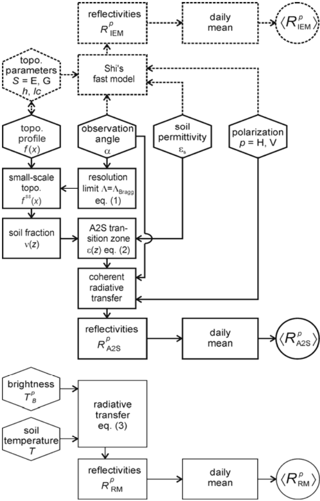
Fig. 1. Illustration of the procedures applied for deriving rough surface reflectivities R_M^p ( p = H, V ; M = \text{IEM, A2S, RM} ). Hexagons indicate model inputs. Reflectivities R_{\text{IEM}}^p computed with the IEM model (dashed-line boxes) require the topography parameters h, lc, S = E, G (either pre-set or derived from topography profiles f(x) ). Reflectivities R_{\text{A2S}}^p computed with the A2S model (solid-line boxes) directly use f(x) as input. Reflectivities R_{\text{RM}}^p (thin-line boxes) are derived from measured brightness and soil temperatures T_B^p and T .
