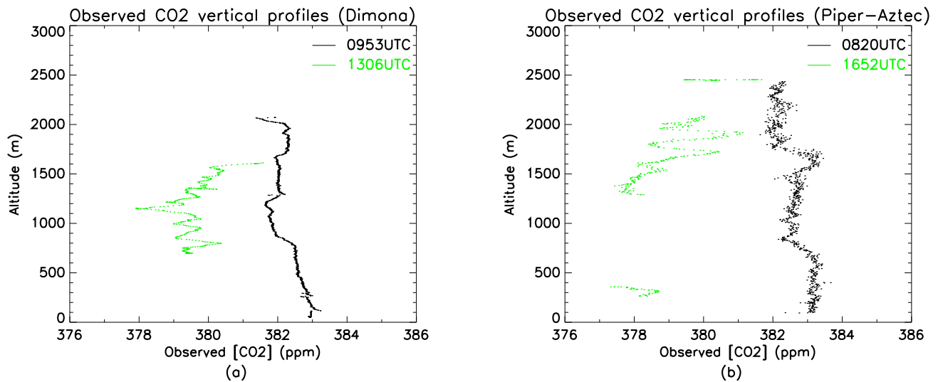
Fig. 10. Vertical profiles of CO 2 concentration observed by: the Dimona aircraft at 09:53 over the ocean (black) and 13:06 UTC inland (green) (a) ; and the Piper-Aztec aircraft at 08:20 UTC over the ocean (black) and 16:52 UTC inland (green) (b) .
