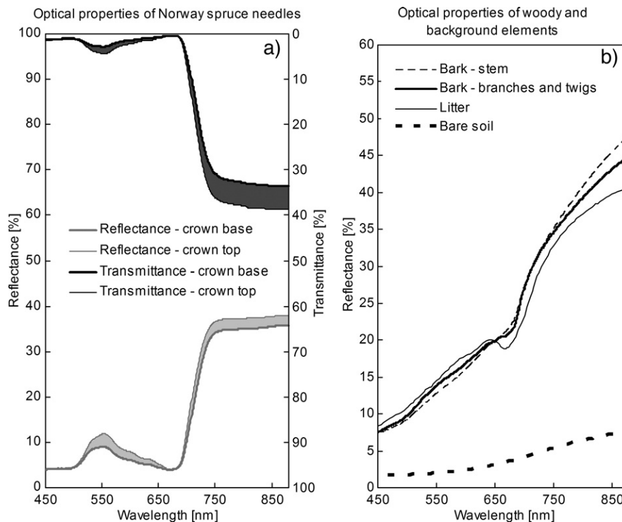
Fig. 4. Measured optical properties (hemispherical–directional reflectance and transmittance) of the surfaces used to parameterize the DART simulations: a) ranges of the Norway spruce needle optical properties defined from base to top of the crown, b) optical properties of woody elements (bark of stem, branches and twigs) and background (litter and bare soil).
