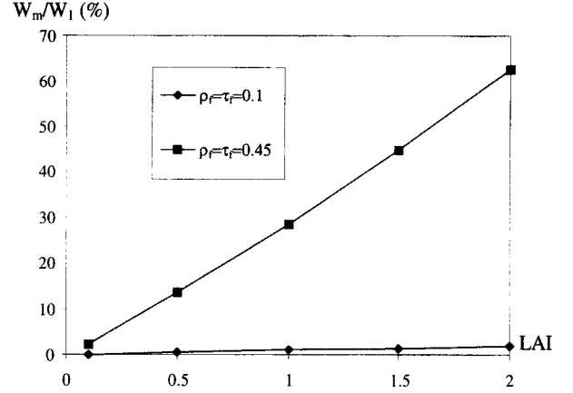
Figure 5. Ratio W_M(\Delta l_i, \Omega_s \rightarrow \Omega_v) / W_1(\Delta l_i, \Omega_s \rightarrow \Omega_v) of a leaf cell as a function of cell LAI. Two cases are considered: \omega_d = 0.9 and \omega_d = 0.2 . The LAD is spherical and leaf specular reflectance is neglected.
