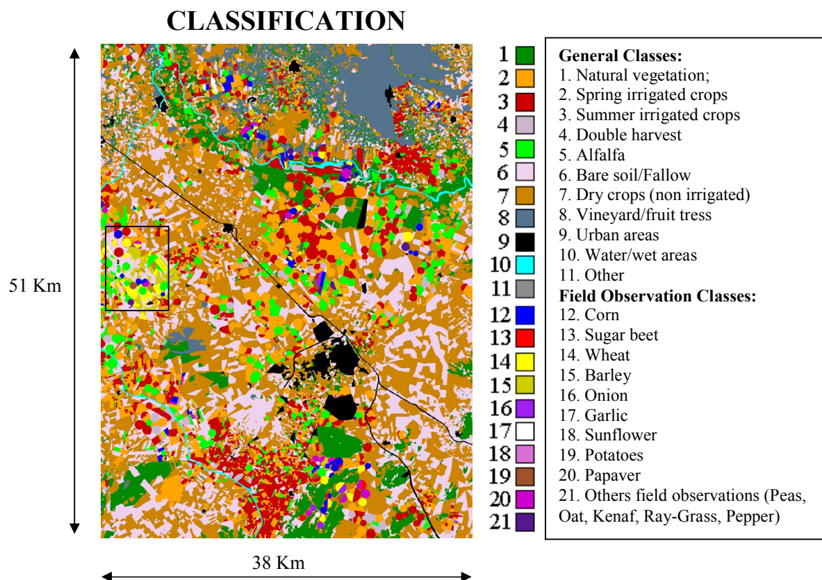
Figure 2. Land use map of the study area. Classes 12 to 21 are local refinements of classes 2 to 7. The black rectangle corresponds to Figure 1.
